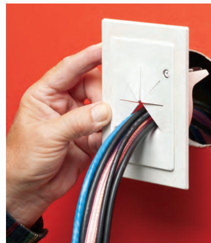
...through the slotted opening in CE1RP. Insert into hole. Level, straighten the bracket.
