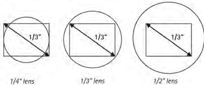
Examples of different lenses mounted onto a 1/3-inch image sensor
