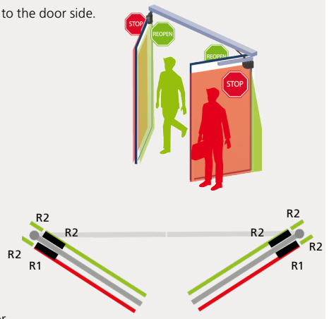
RELAY 1: STOP-impulse on the opening side of the door.
