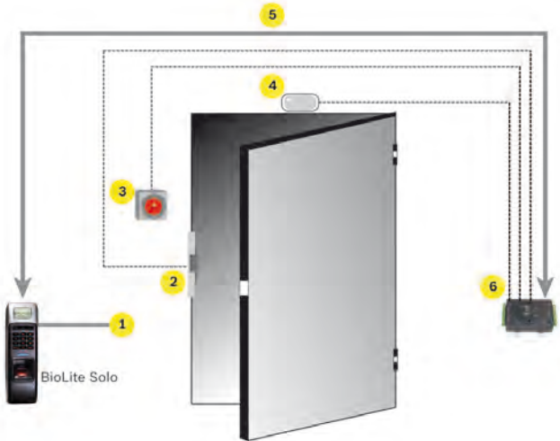
1 = Power supply; 2 = Door lock; 3 = Exit button; 4 = Door sensor; 5 = RS485 secure communication; 6 = Secure I/O module
