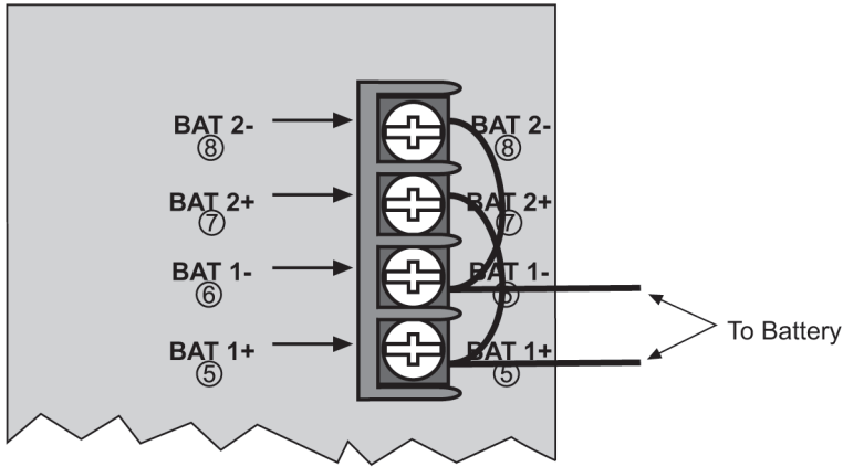
Figure 4.2: Jumper locations for single-battery installations
