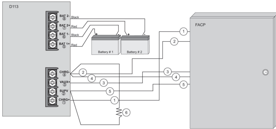
Figure 4.1: Wiring the module
