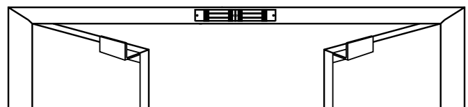
Double Lock, Inswing Door Center Mounted To Header Face With Adjustable Top Jamb "Z" Brackets
