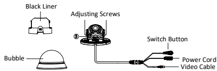
Figure 1-10 Overview of Type VI Camera
