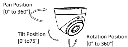
Figure 2-11 3-Axis Adjustment
