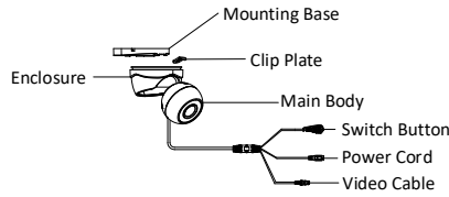
Figure 1-2 Overview of Type I Camera
