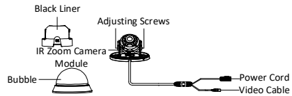
Figure 1-9 Overview of Type VI Camera
