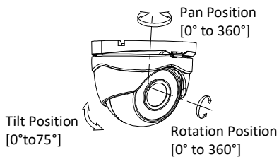
Figure 2-4 3-Axis Adjustment
