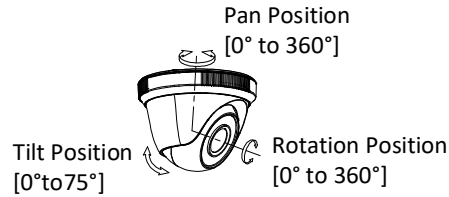
Figure 2-7 3-Axis Adjustment
