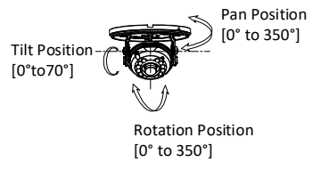
Figure 2-14 3-Axis Adjustment
