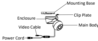
Figure 1-1 Overview of Type I Camera
