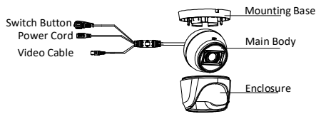
Figure 1-7 Overview of Type IV Camera
