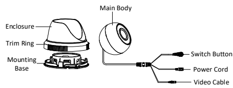
Figure 1-4 Overview of Type II Camera
