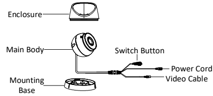
Figure 1-6 Overview of Type III Camera
