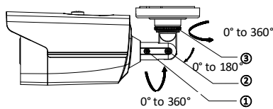
Figure 2-6 3-Axis Adjustment
