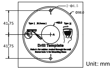
Figure 2-14 Drill Template
