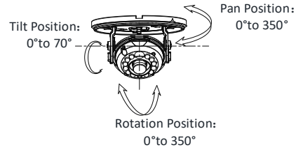
Figure 2-16 3-axis Adjustment
