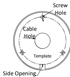
Figure 2-1 Drill Template
