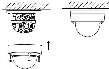
Figure 2-11 Bubble Reinstallation
