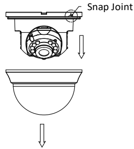
Figure 2-13 Remove the Bubble
