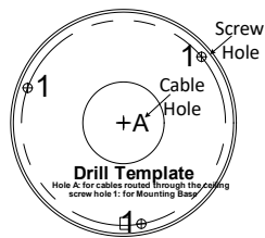
Figure 2-7 Drill Template
