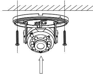
Figure 2-15 Attach the Mounting Base to the Ceiling
