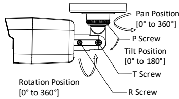
Figure 2-3 3-axis Adjustment
