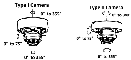
Figure 2-4 3-Axis Adjustment
