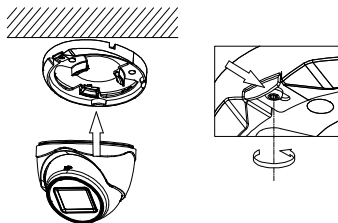
Figure 2-11 Install the Turret Camera
