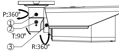
Figure 2-3 3-axis Adjustment
