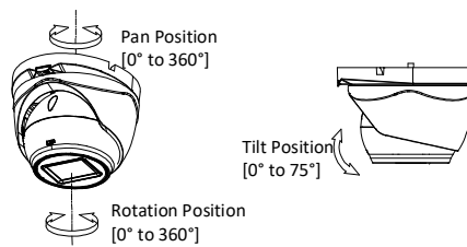
Figure 2-12 3-axis Adjustment
