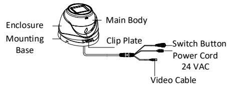
Figure 1-2 Overview of Type II Camera
