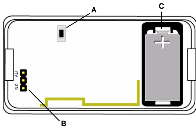
Figure 1 EN1224/EN1224-ON components
