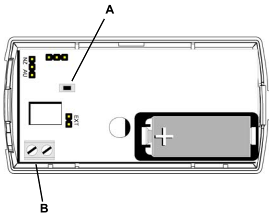
Figure 1 EN1751 components
