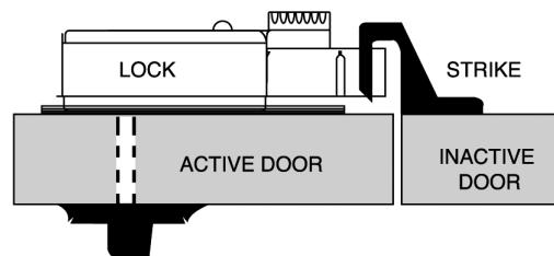
TYPE 9 Part# 114006
