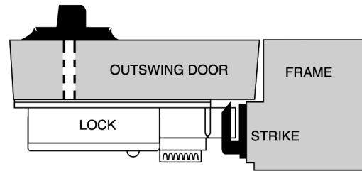
TYPE 2 Part# 114004
