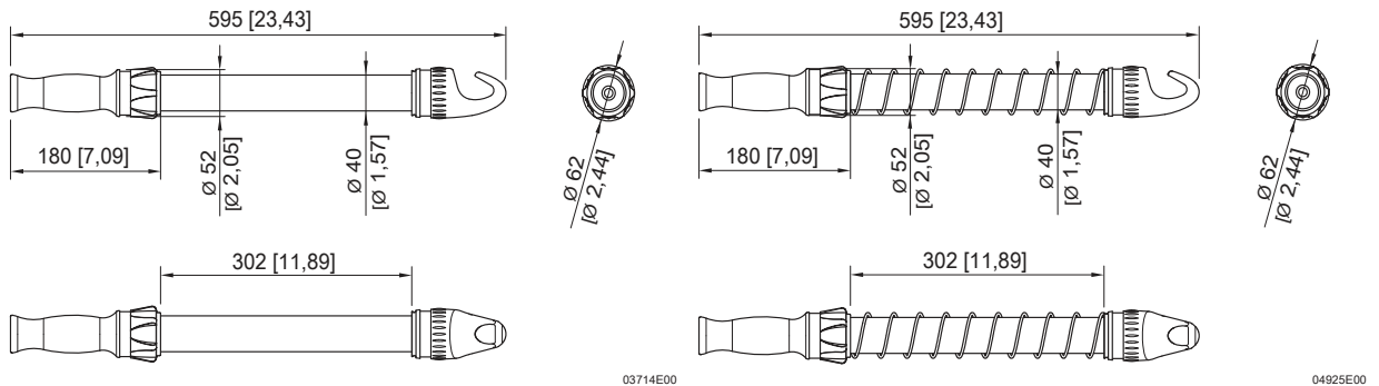
Inspection light without wire guard
