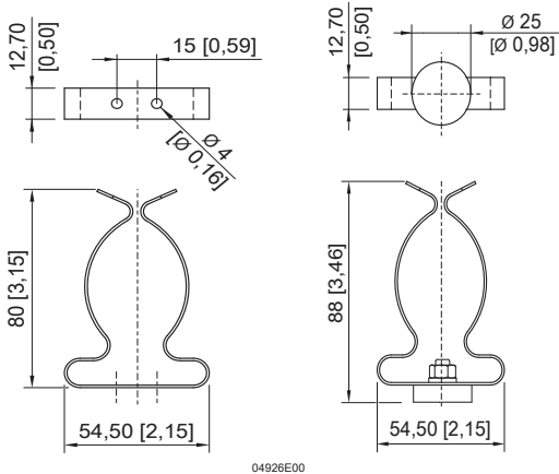
Mounting bracket
