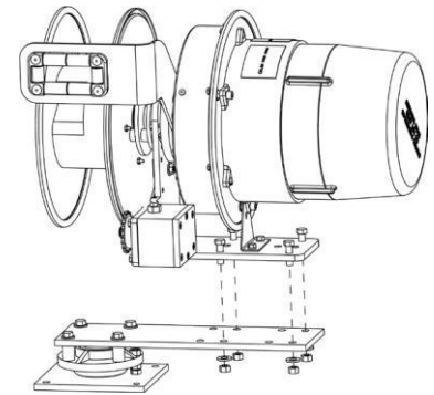
Reel with Pivot Base
