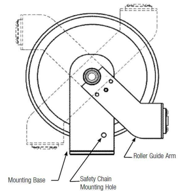
Roller Guide Locations
