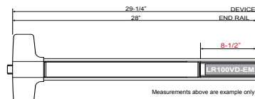
32" Opening (36" Device Modified for 32" Opening)
