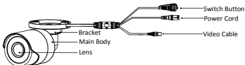
Figure 1-2 Overview of Type I Camera
