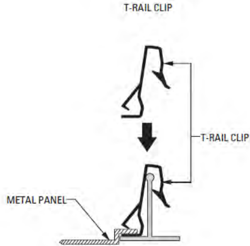
Figure 1. Attaching the T-Rail Clips
