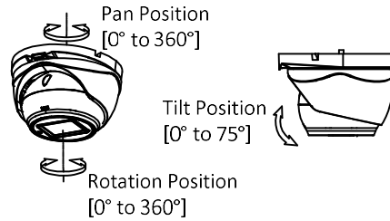
Figure 2-11 3-axis Adjustment
