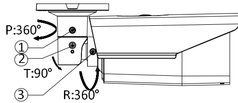
Figure 2-3 3-axis Adjustment
