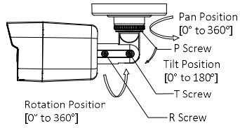
Figure 2-3 3-axis Adjustment
