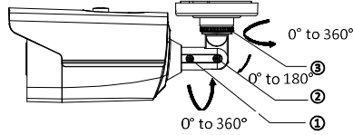
Figure 2-10 3-Axis Adjustment
