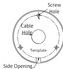
Figure 2-8 Drill Template
