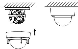
Figure 2-20 Bubble Reinstallation
