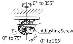
Figure 2-19 Type I Camera 2-Axis Adjustment
