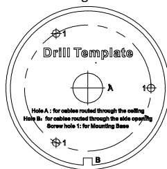
Figure 2-2 Drill Template
