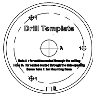
Figure 2-7 Drill Template
