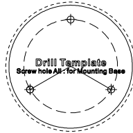
Figure 2-12 Drill Template
