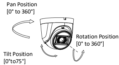
Figure 2-10 3-axis Adjustment
