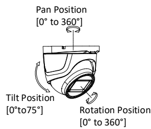
Figure 2-15 3-axis Adjustment
