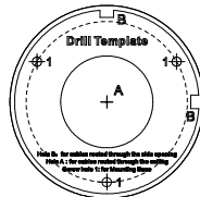
Figure 2-4 Drill Template
