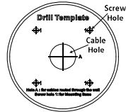
Figure 2-13 Drill Template of the Junction Box
