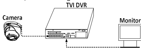
Figure 3-1 Connection
