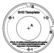
Figure 2-1 Drill Template
