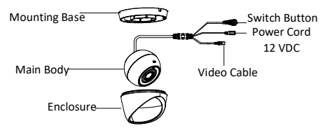
Figure 1-7 Overview of Type VII Camera
