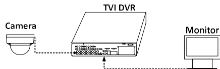
Figure 2-1 Connection
