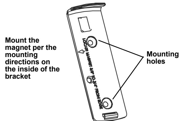
Figure 2 Mount the bracket
