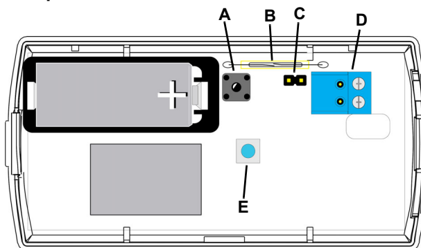
Figure 1 Door/window with reed switch internal components
