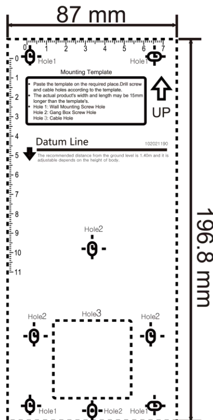
Figure 3-4 Mounting Template
