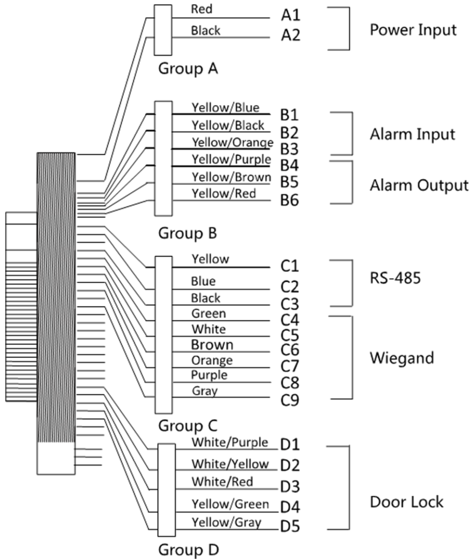
Figure 4-1 Terminal Diagram
