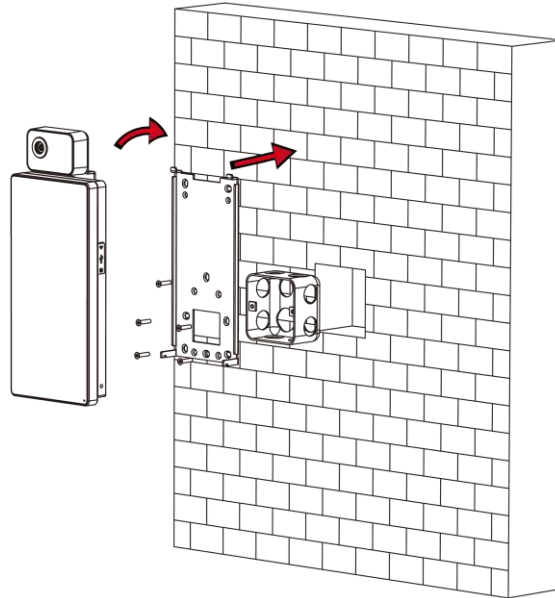
Figure 3-2 Install Device
