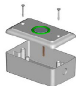
Figure 6: MP-06 Mount
