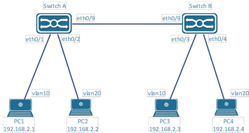
Figure 3-7 network topology diagram
