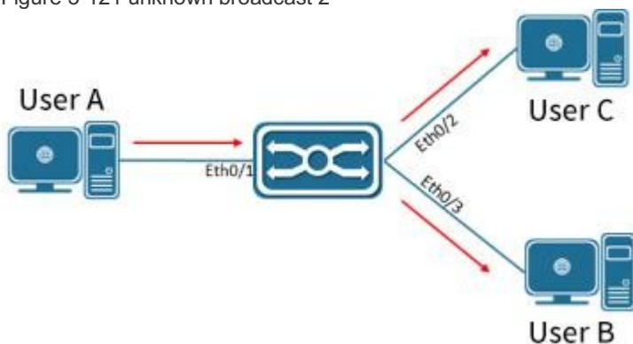
Figure 3-121 unknown broadcast 2
