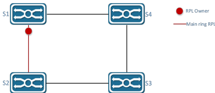
Figure 3-16 ERPS single-loop model
