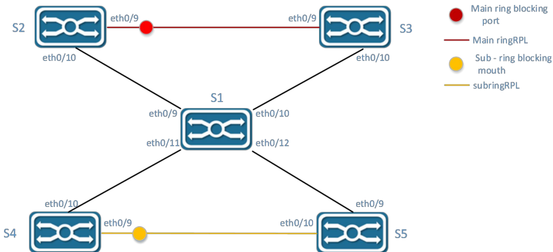
Figure 3-33 network topology
