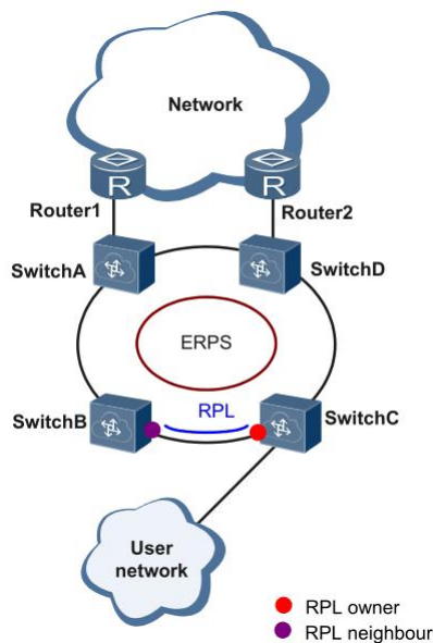
Figure 3-13 typical ERPS networking
