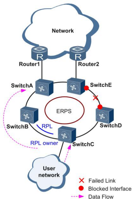
Figure 3-15 ERPS link failure
