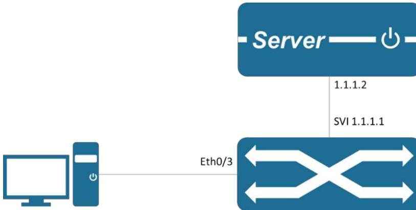
Figure 4-41 Typical MAC Authentication Networking Diagram
