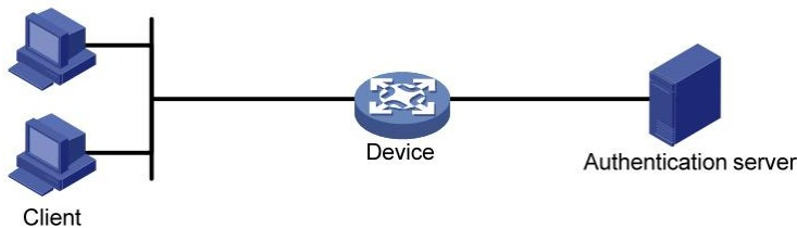
Figure 4-26 802.1x Architecture
