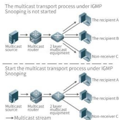
Figure 3-83 how IGMP Snooping works
