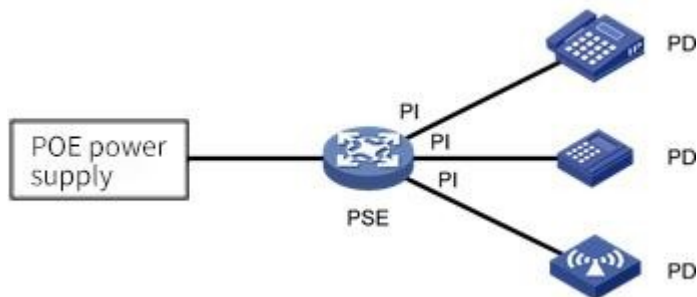
Figure 2-27 PoE system
