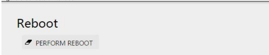
Figure 5-36 restart interface
