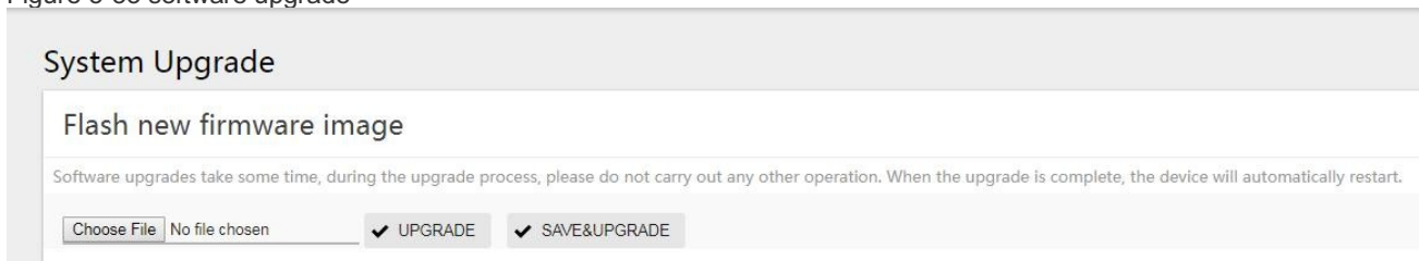
Figure 5-33 software upgrade
