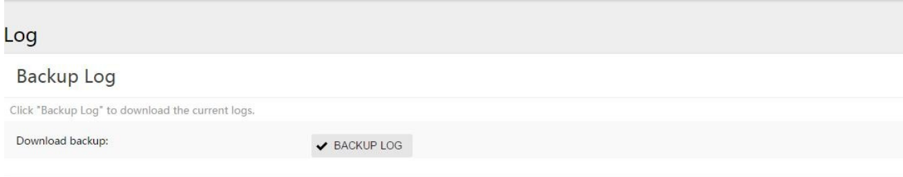
Figure 5-35 log/diagnostic interface
