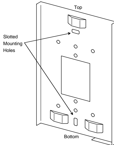
Figure 2. Mounting Bracket
