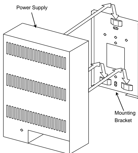
Figure 3. Mounting the Power Supply
